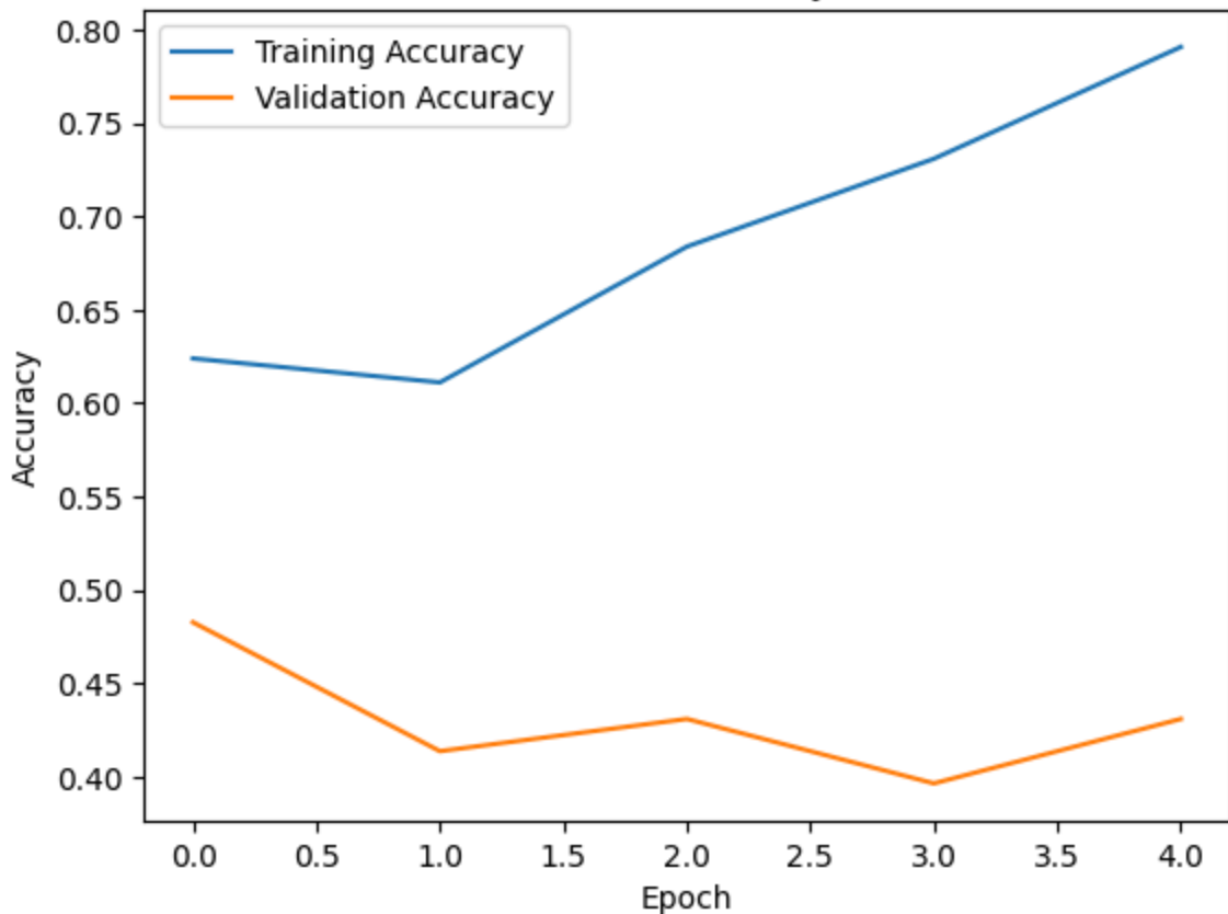
Model Accuracy
